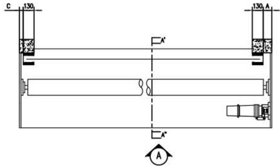
PLAN OF MOTORISED INSULATED FIRE STEEL SHUTTER (IFSS)
