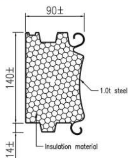
SLAT PROFILE
